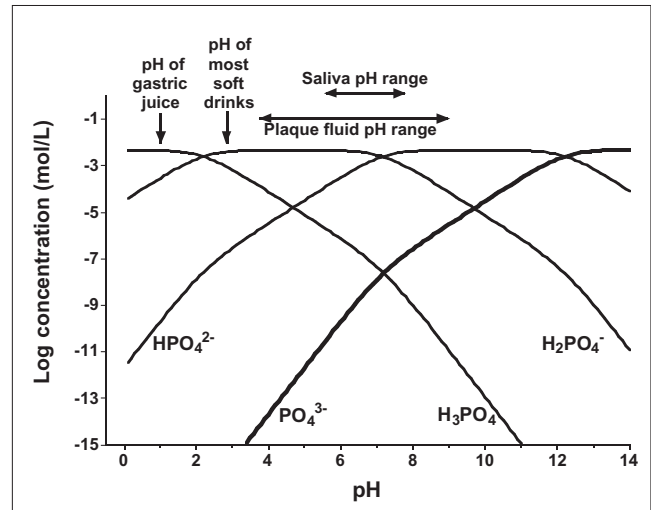
Figure 1: The effect of pH on the concentrations of the various inorganic phosphate species in saliva containing a total phosphate concentration of 5 \times 10^{-3} mol/L. There is a marked fall in the concentration of PO_4^{3-} (thick line) as the pH is reduced.
